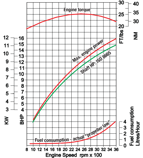
FUEL CONSUMPTION BASED ON PROPELLER BEING MATCHED AT FULL SPEED.
